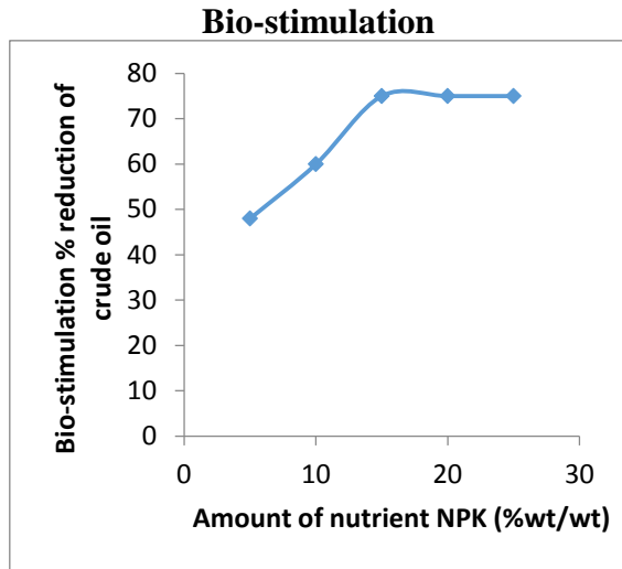
Fig 2: Effect of amount of nutrient on percentage reduction of crude oil.
