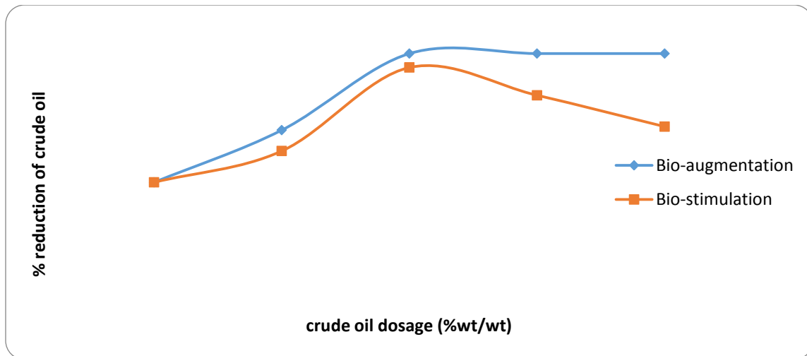
Fig 3: Effect of crude oil dosage on percentage reduction of crude oil.
