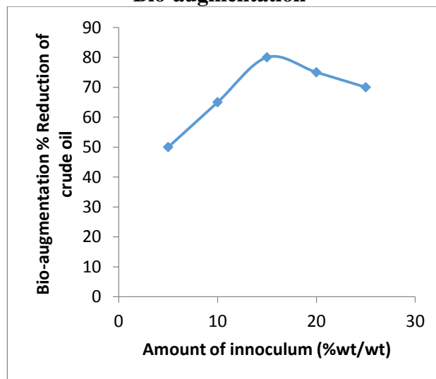
Fig 1; Effect of amount of inoculums on reduction of crude oil.
