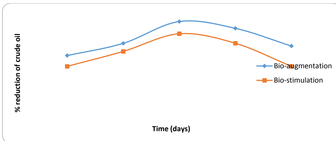
Fig 4: Effect of time on percentage reduction of crude oil.
